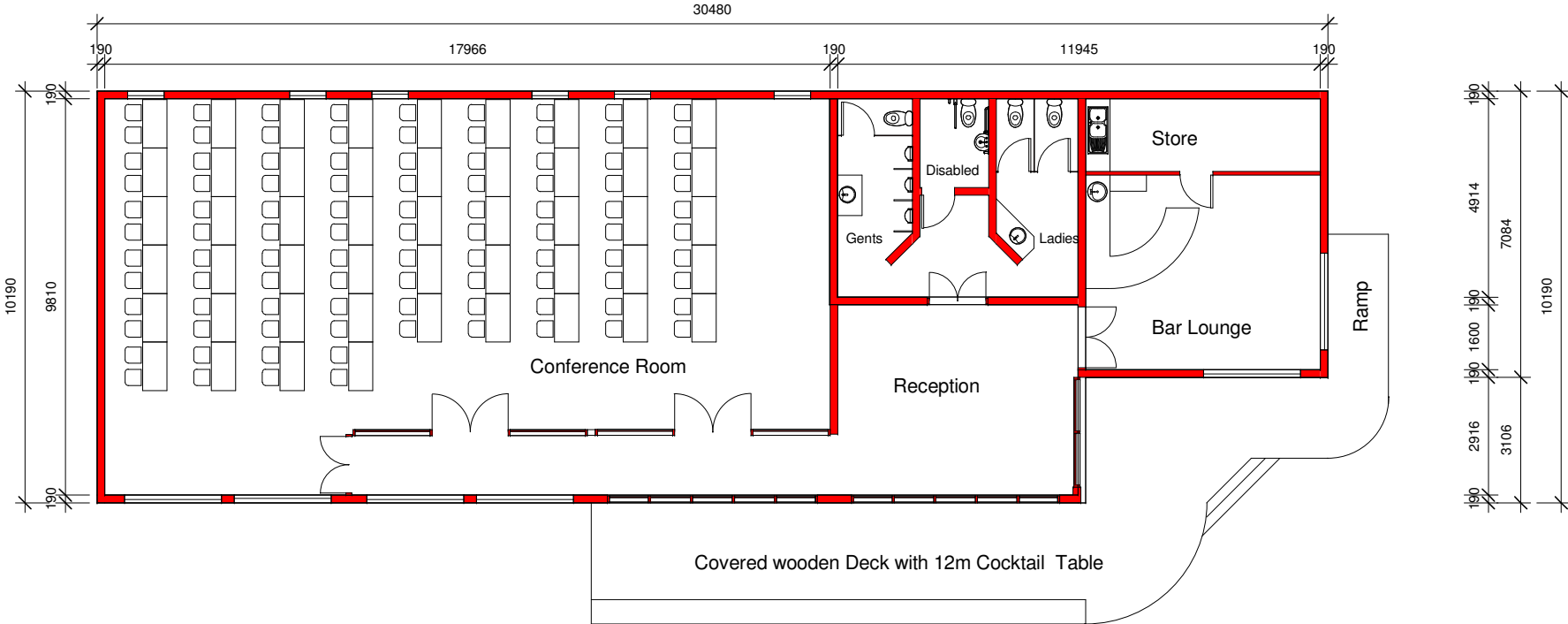
1 Ground Floor Plan 1 : 100
